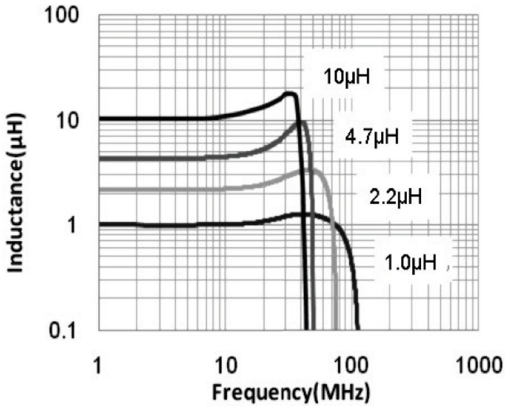
Inductance vs. Frequency Characteristics
